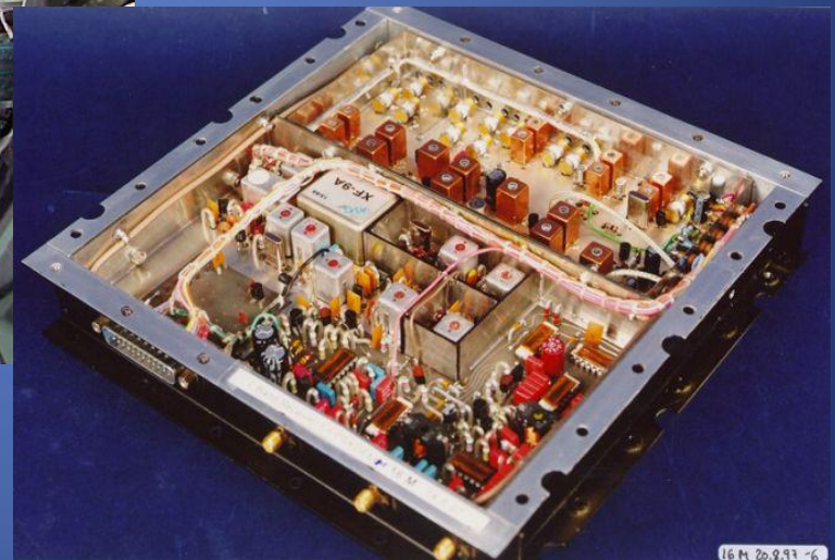
PHASE 3D Satellite - Command Receiver
